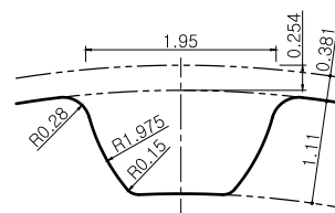
치형: S3M / Pitch: 3mm
