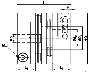
Size : 12C~47C & 80C~100C
