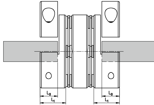
Side-clamp Split
