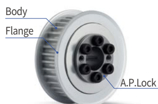
A.P.Lock Type (SPA□)
