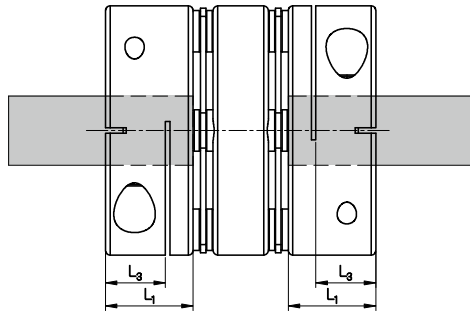
Side-clamp
