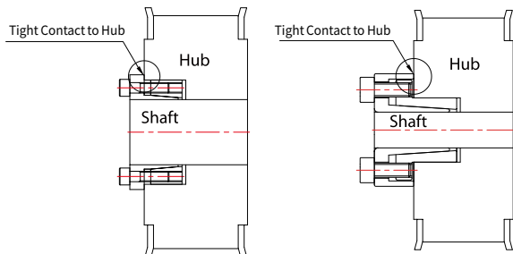
▲ SAPL-B Series (Example)
