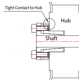
▲ SAPL-T Series (Example)
